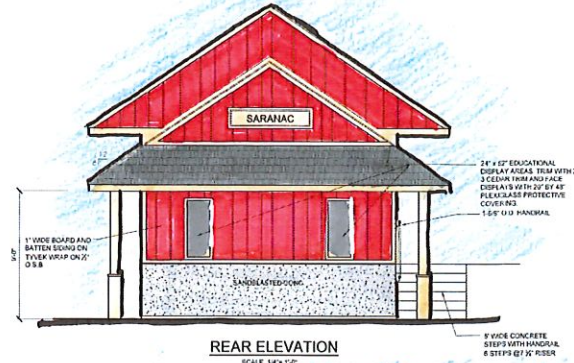
REAR ELEVATION SCALE: 1/4\"/>
