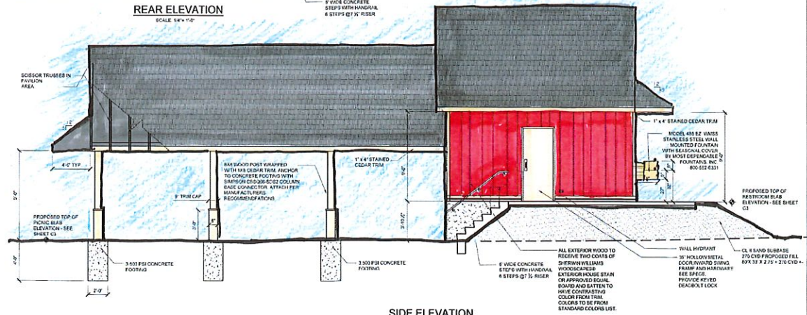
SIDE ELEVATION SCALE: 1/4\"/>
