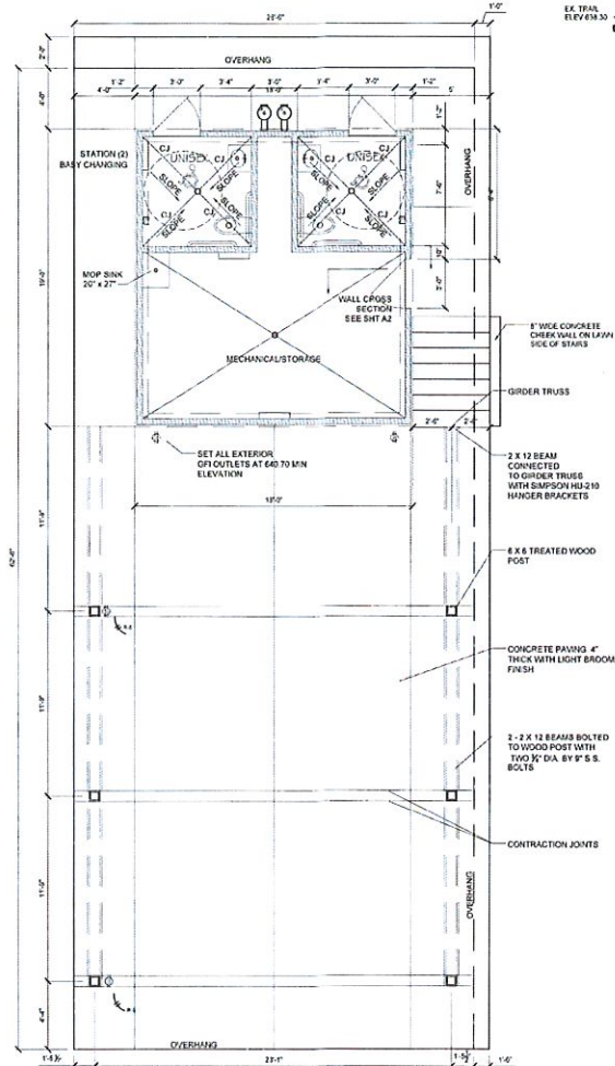
FLOOR PLAN SCALE: 1/4\"/>
