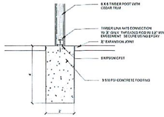
TIMBER CONCRETE CONNECTION NOT TO SCALE
