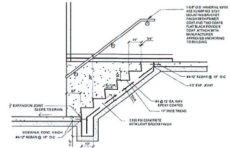
CONCRETE STEP DETAIL NOT TO SCALE
